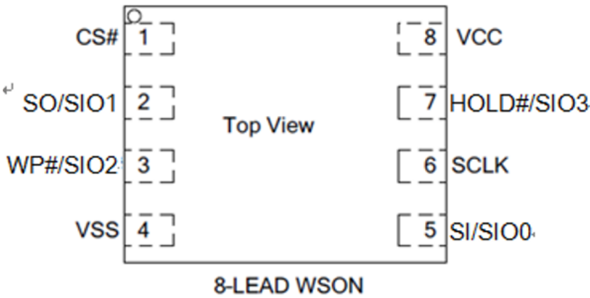
Figure 6.1 Pin Configuration
