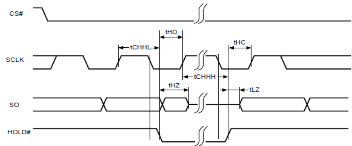
Figure 4.3 Hold Timing
