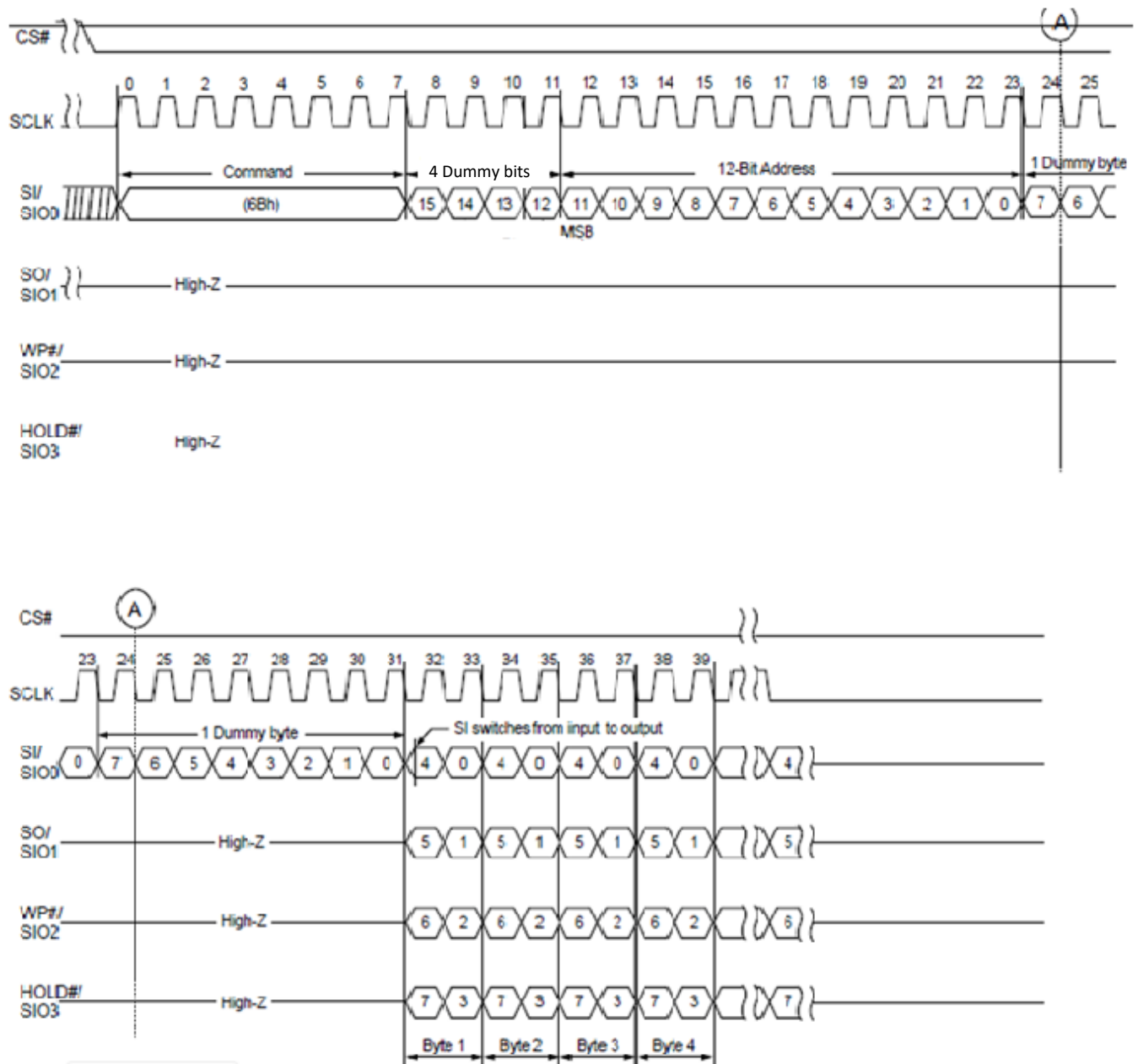
Figure 3.8 Read From Cache x4
