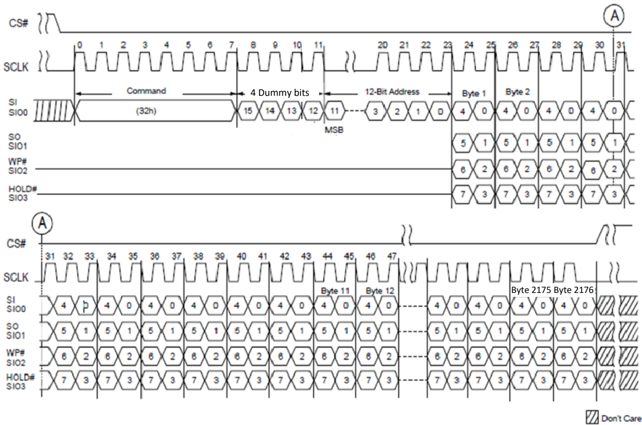
Figure 3.11 Program Load x4 (32h)
